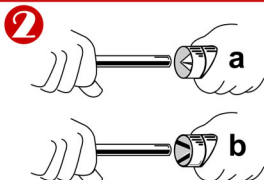
2. (2a) Ream, then de-burr (2b)
