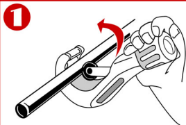
1. Cut the pipe or tubing
