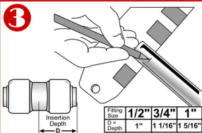
3. Mark the insertion depth
